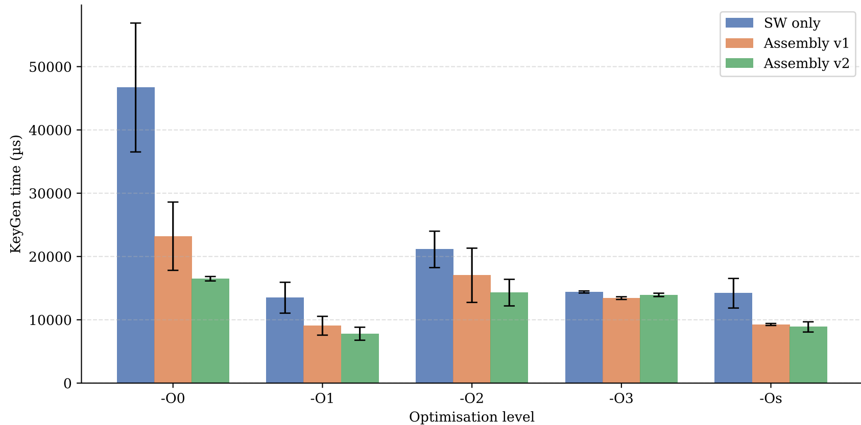
KeyGen: SW-only vs Assembly v1 vs Assembly v2 under QEMU (100 runs, error bars = 1 std dev)
