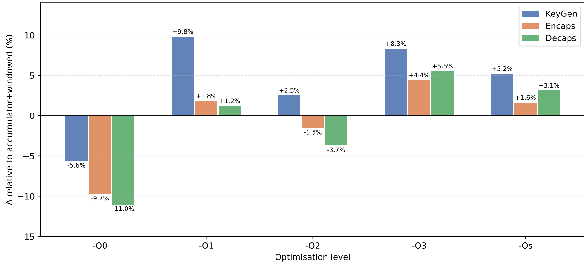
Paired-load+windowed vs accumulator+windowed (positive = paired-load slower, negative = paired-load faster)
