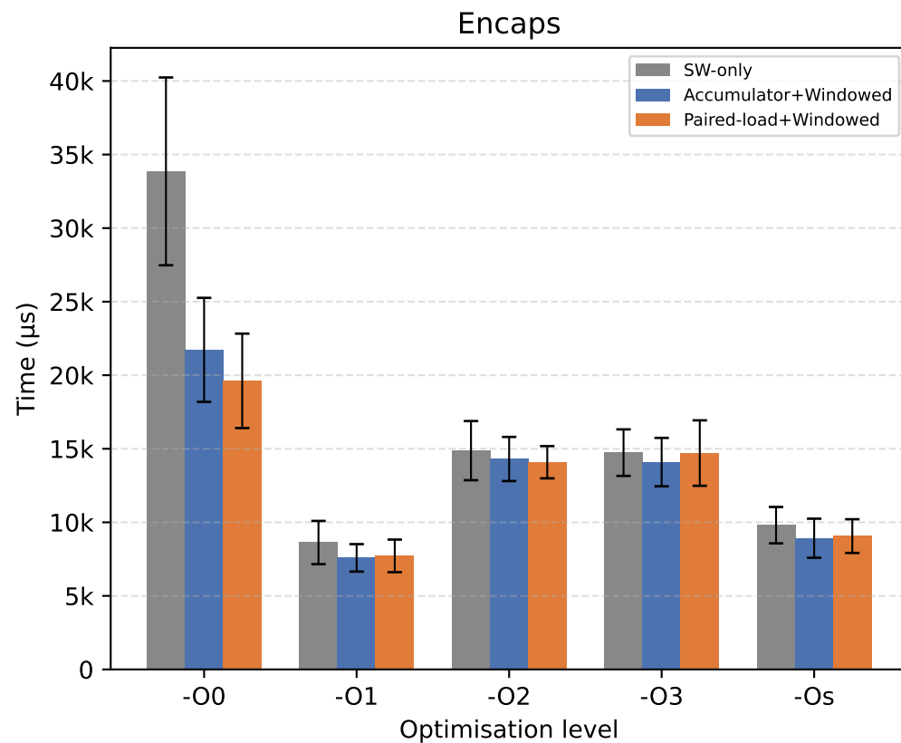
Wall-clock time: SW-only vs both combined assembly configurations (100 runs, error bars = 1 std dev)
