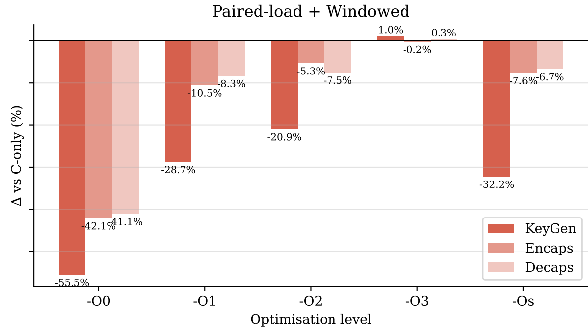
Improvement over C-only baseline (negative = faster)
