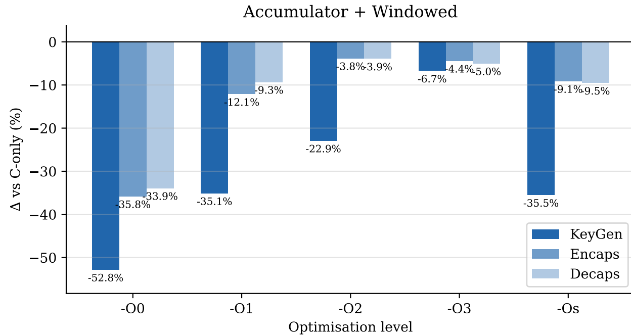
Improvement over C-only baseline (negative = faster)
