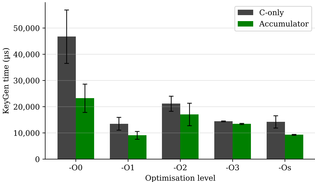
KeyGen: C-only vs Accumulator under QEMU (100 runs, error bars = 1 std dev)
