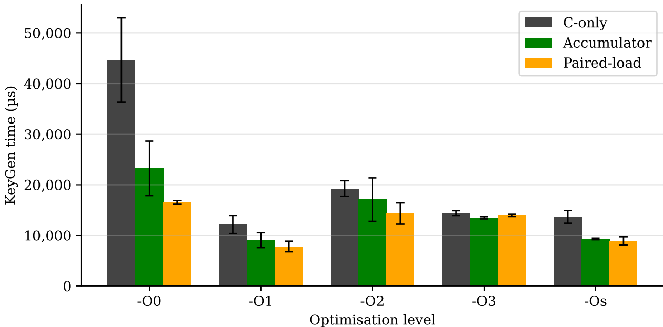
KeyGen: C-only vs Accumulator vs Paired-load under QEMU (100 runs, error bars = 1 std dev)
