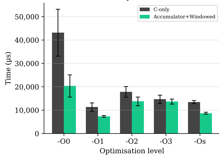
KeyGen
