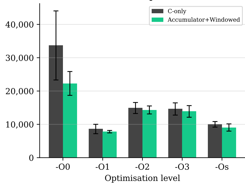
Decaps
