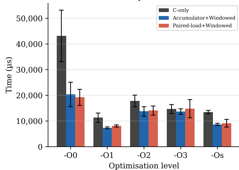
KeyGen
