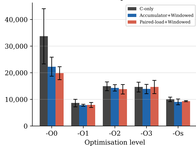
Decaps
