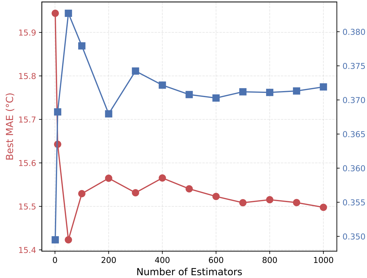
C: Best Performance vs N_Estimators
