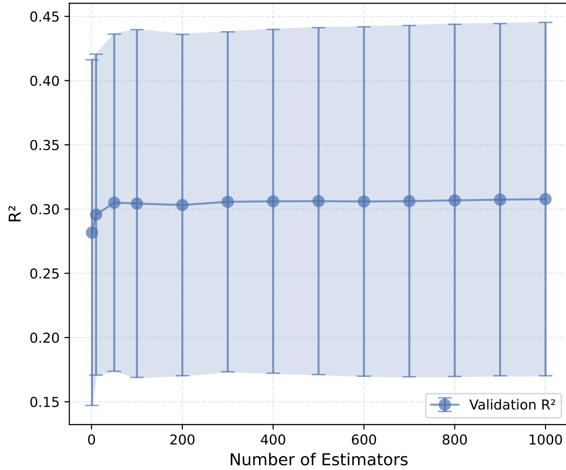
B: Average R 2 vs N_Estimators
