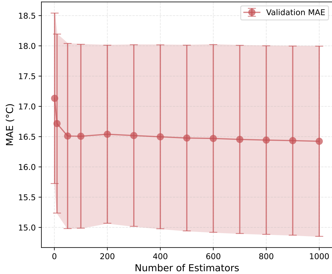
A: Average MAE vs N_Estimators
