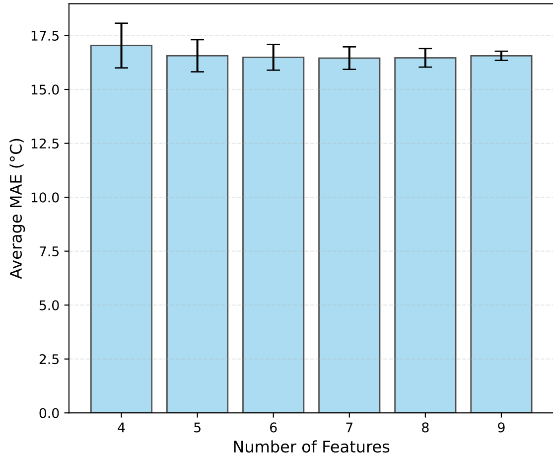
D: Performance by Feature Count
