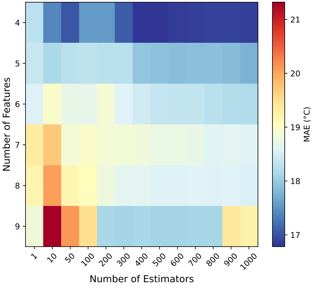
E: Validation MAE Heatmap
