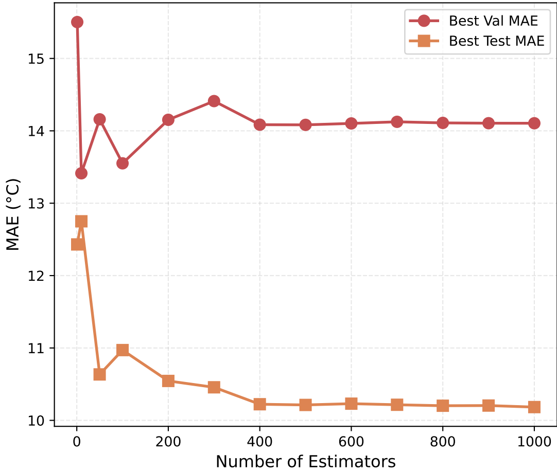
C: Best Performance vs N_Estimators
