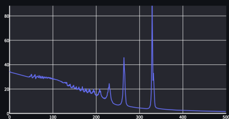
Loss Graph
