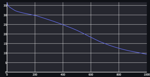
Loss Graph
