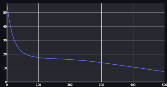
Loss Graph
