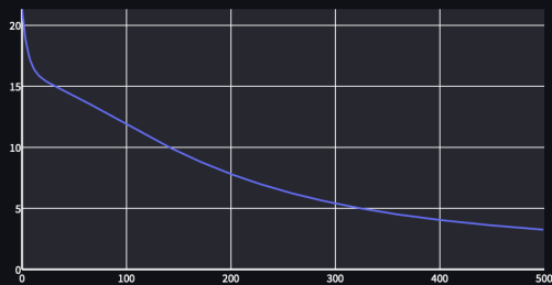
Loss Graph
