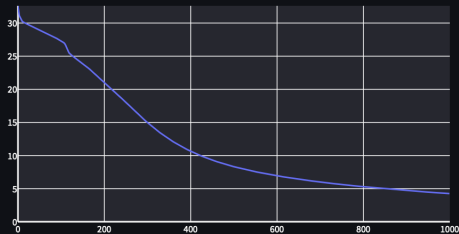
Loss Graph
