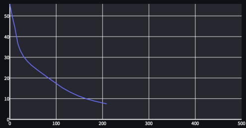
Loss Graph
