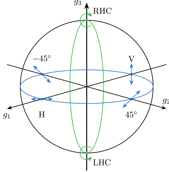
Figure 2.1: Representation of the polarization state on the Poincaré sphere. Fully polarized waves lie on the surface ( DOP = 1 ), while partially polarized states lie within the volume ( DOP < 1 ). The axes g_1, g_2, g_3 correspond to linear, linear-diagonal, and circular polarizations, respectively.
