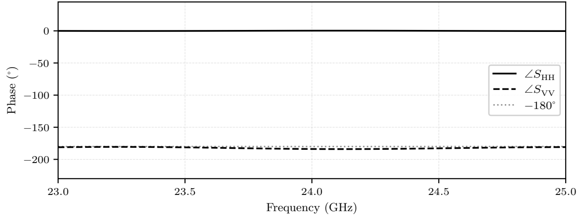
(b) Phase response showing the \pi phase difference between co-polarized channels.
