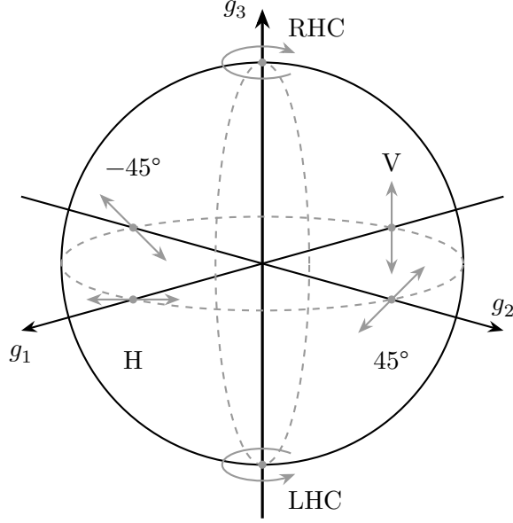
Figure 2.1: Representation of the polarization state on the Poincaré sphere.
