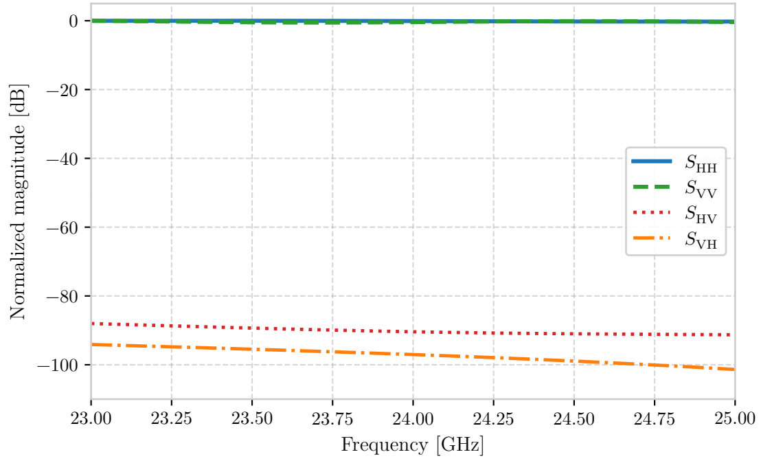
(a) Normalized magnitude response showing strong co-polar returns and low cross-polar leakage.
