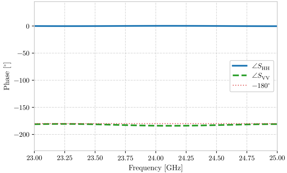
(b) Phase response showing the \pi phase difference between co-polarized channels.
