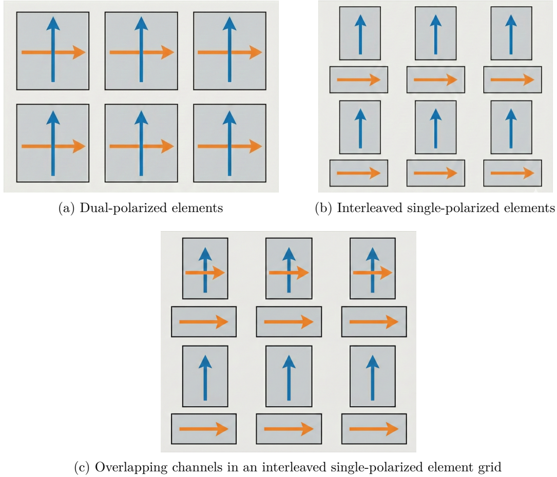
Figure 3.1: Comparison of physical element arrangements for polarimetric MIMO radar.
