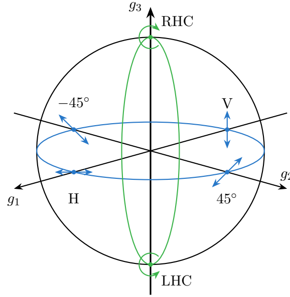
Figure 2.1: Representation of the polarization state on the Poincaré sphere. Fully polarized waves lie on the surface (DOP = 1), while partially polarized states lie within the volume (DOP < 1). The axes g_1, g_2, g_3 correspond to linear, linear-diagonal, and circular polarizations, respectively.
