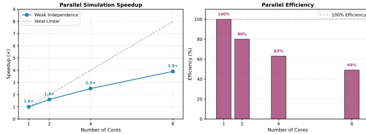
Fig. 2: Parallel simulation speedup on multi-core systems. Baseline: sequential execution. Parallel: weakly independent transitions scheduled concurrently.
