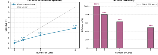
Figure 3: Parallel simulation speedup on multi-core systems. Baseline: sequential execution. Parallel: weakly independent transitions scheduled concurrently.
