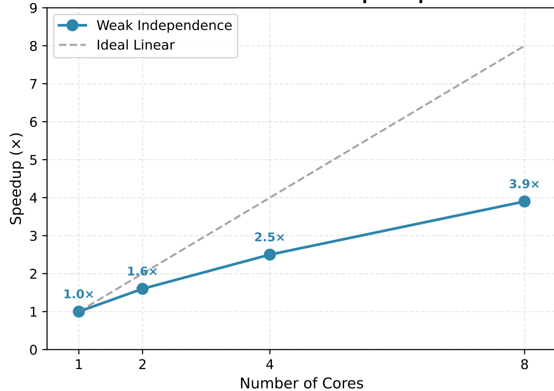
Parallel Simulation Speedup
