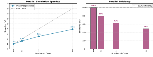
Figure 3: Parallel simulation speedup on multi-core systems. Baseline: sequential execution. Parallel: weakly independent transitions scheduled concurrently.
