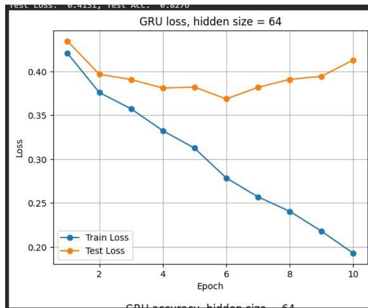
loss - GRU, hidden size = 64
