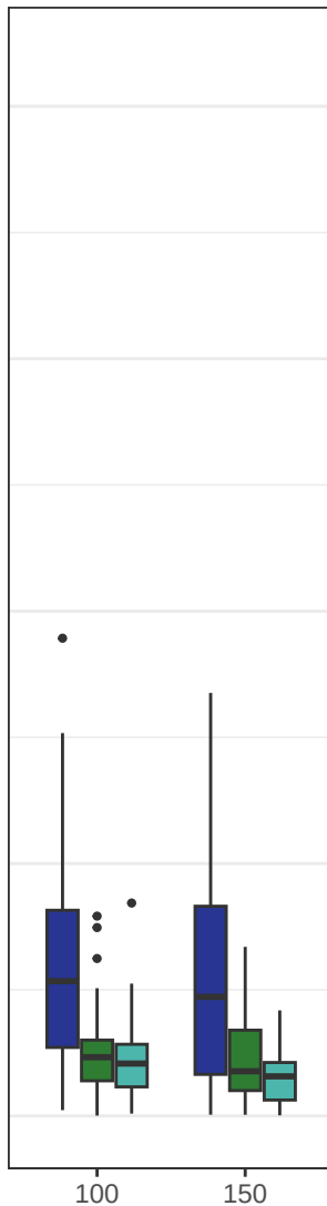
Non-noisy Variables
