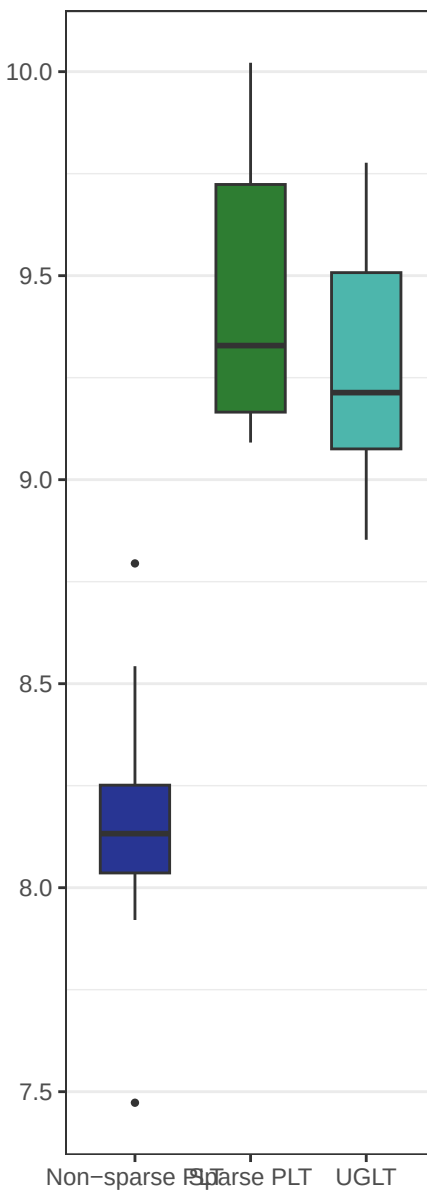
Predictive MSE
