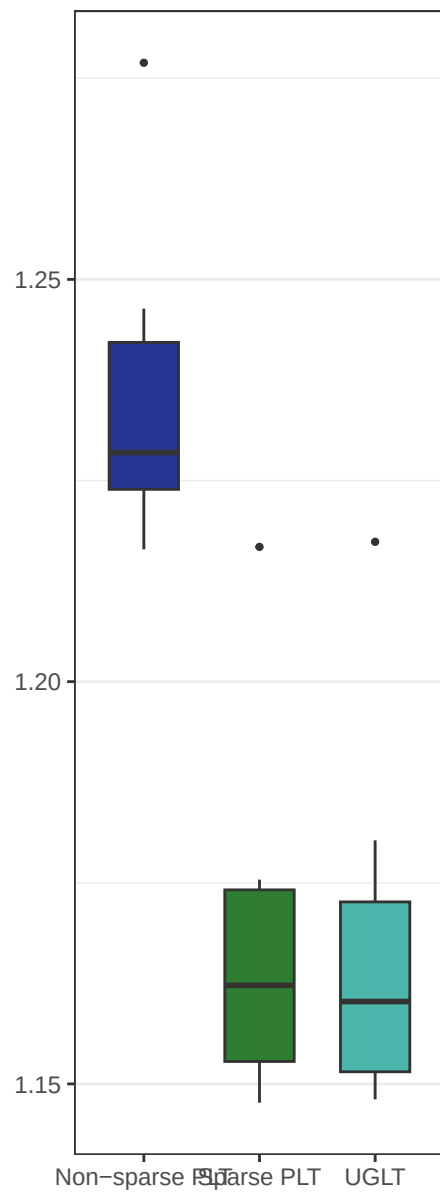
Predictive CRPS
