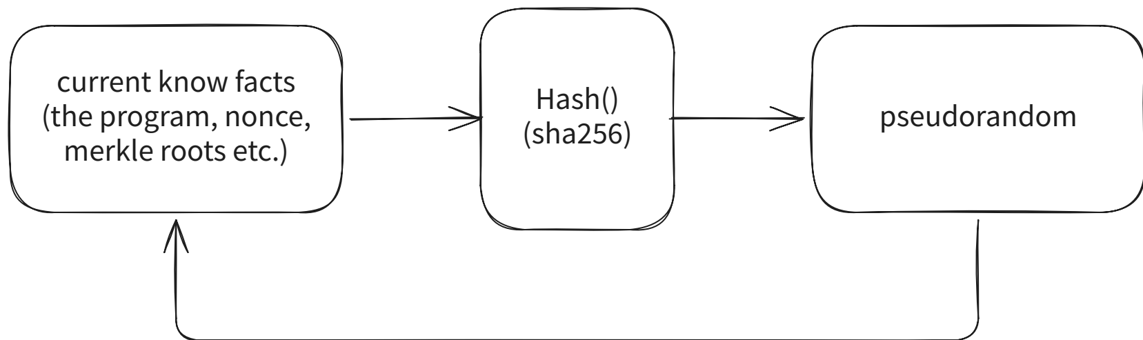
Figure 3: Fiat-Shamir heuristic
