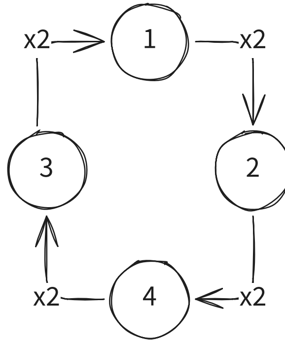
Figure 2: \mathbb{F}_{5/\{0\}} with generator 2
