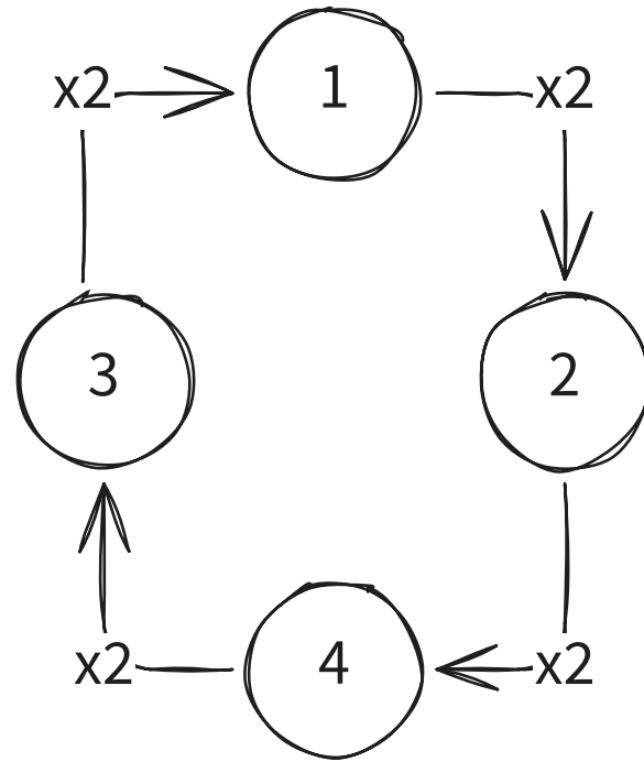
Figure 2: \mathbb{F}_5^* with generator 2
