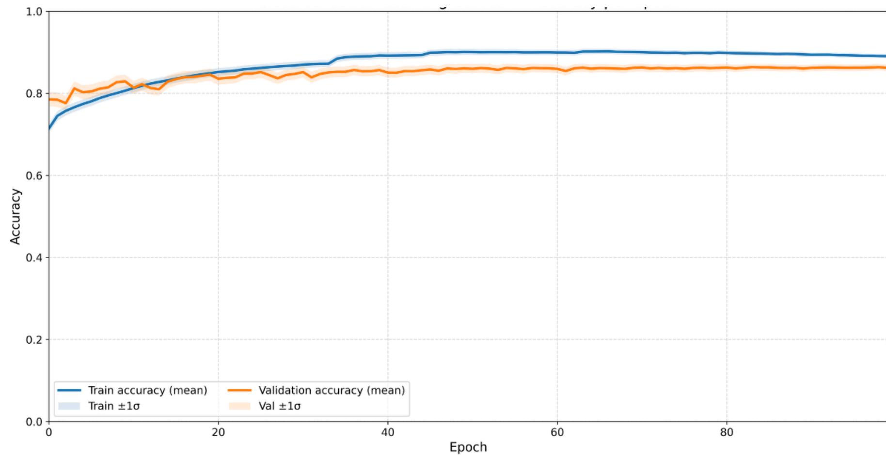
Sleep-EDF78
