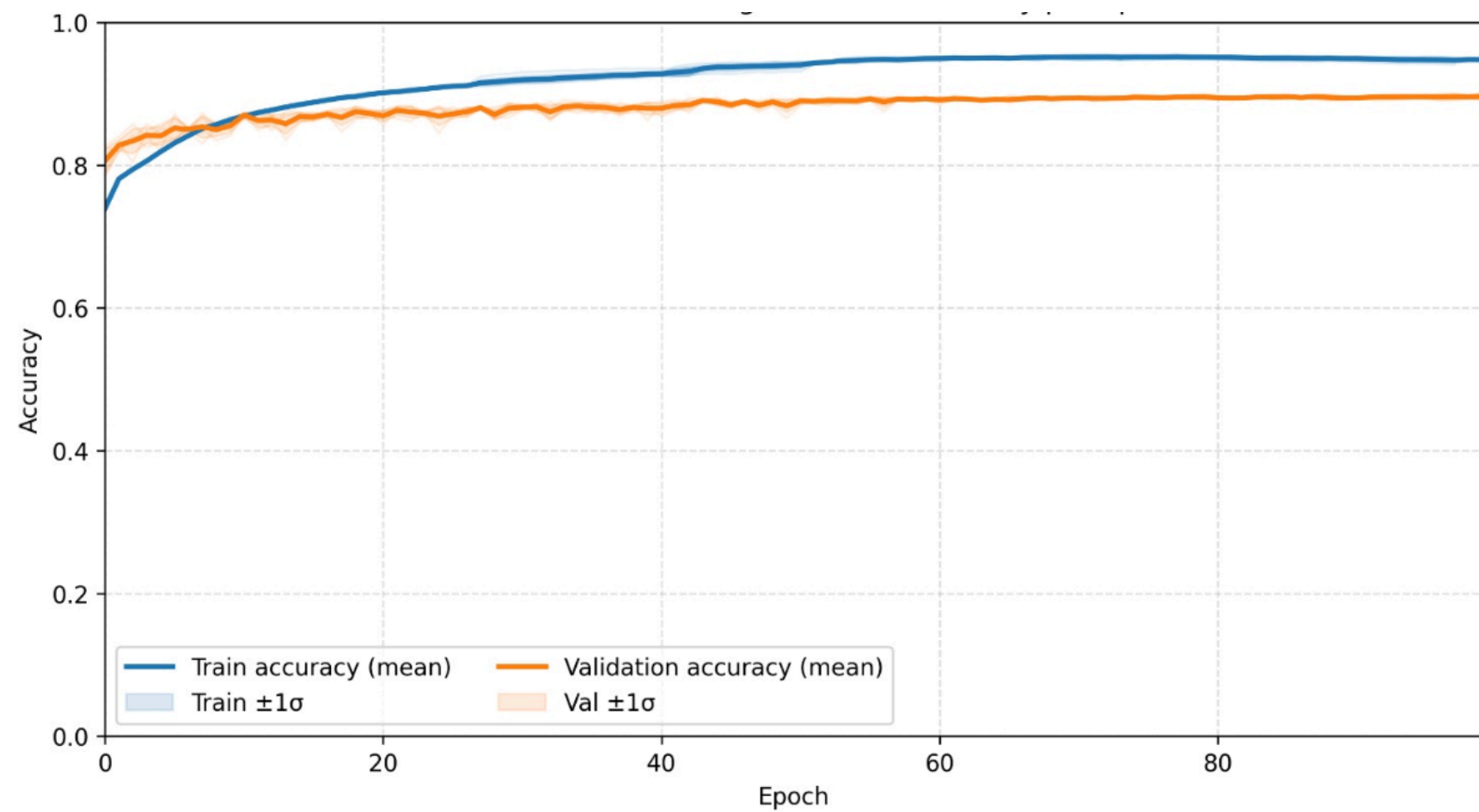
Sleep-EDF20
