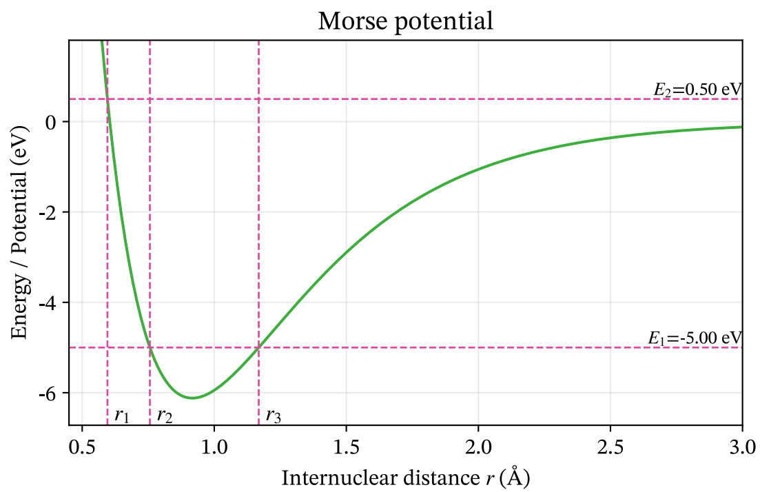
Figure 1.1: Morse potential
