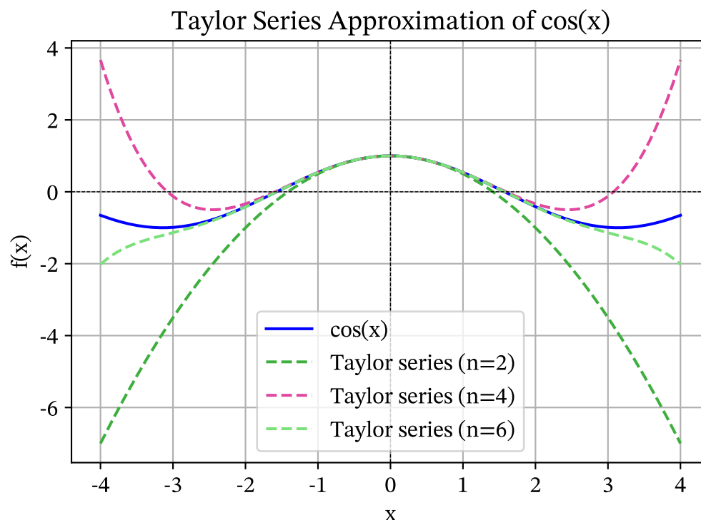
Figure 17.1: Taylor series approximations of \cos(x) about x=0 . The dashed lines show the Taylor polynomials of order 2, 4, and 6.
