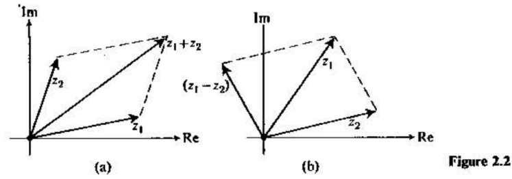
Figure 21.1: The parallelogram rule. (From Butkov.)
