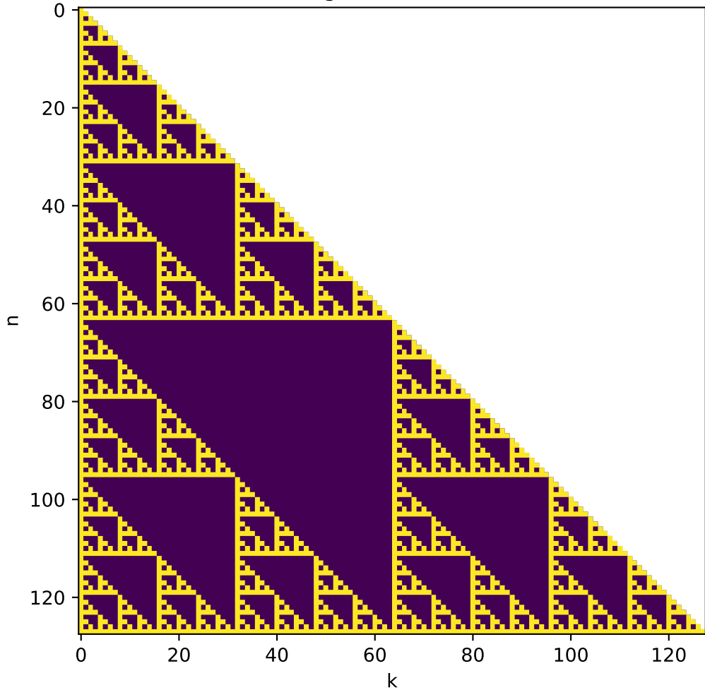
Pascal's Triangle modulo 2 — 128 rows
