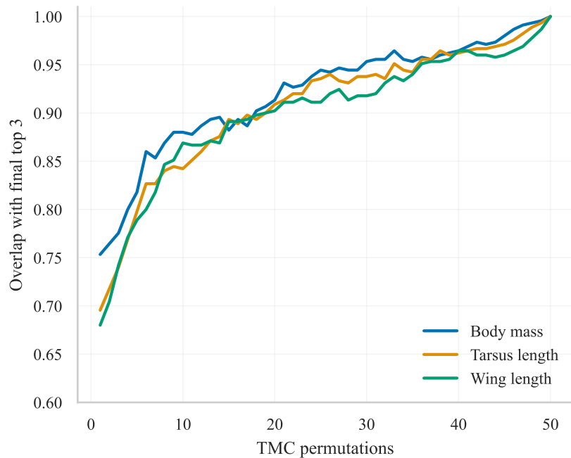
Top-3 stability
