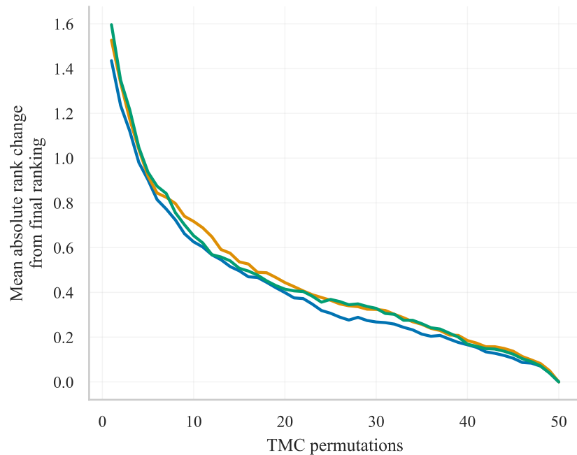
Rank convergence
