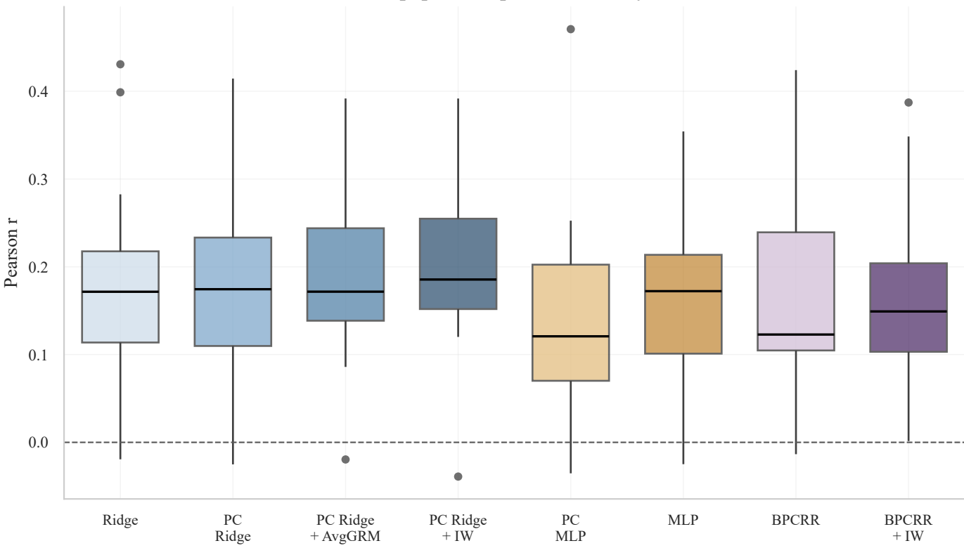
Across-population prediction, Body mass
