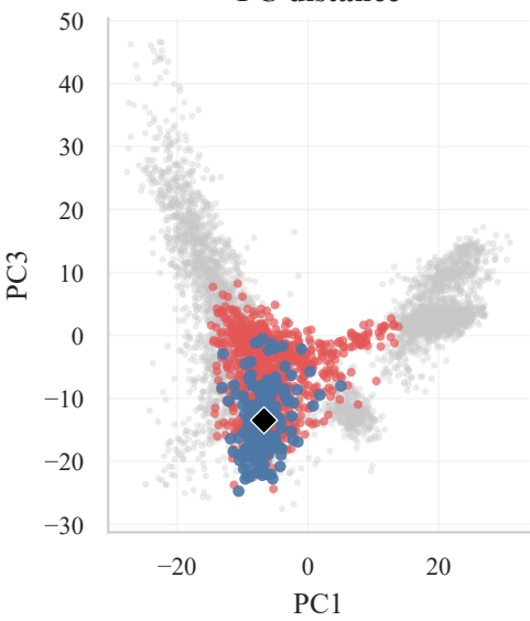
PC distance
