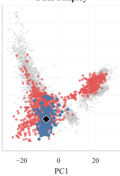
Data Shapley
