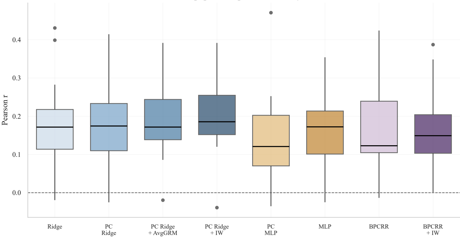
Across-population prediction, Body mass
