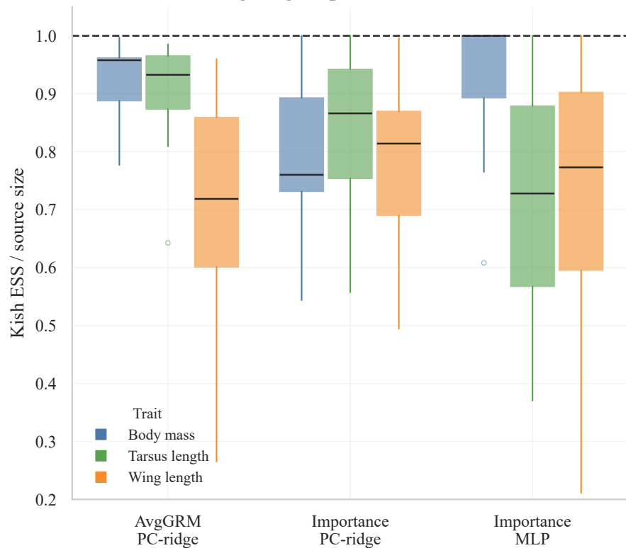
Weighting keeps most of the data
