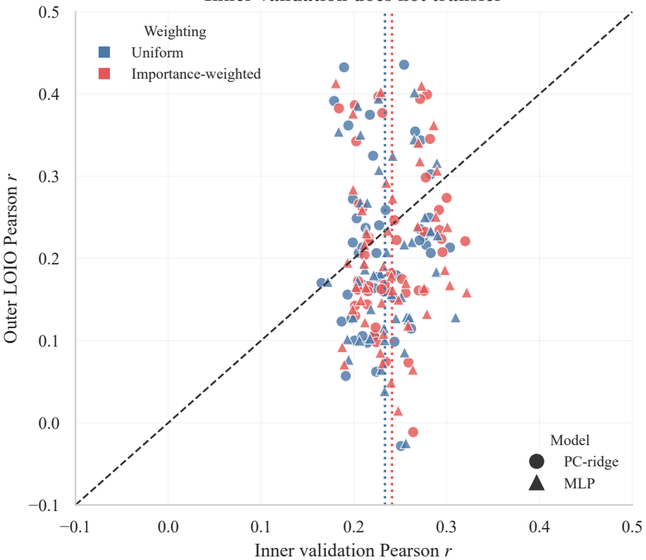
Inner validation does not transfer
