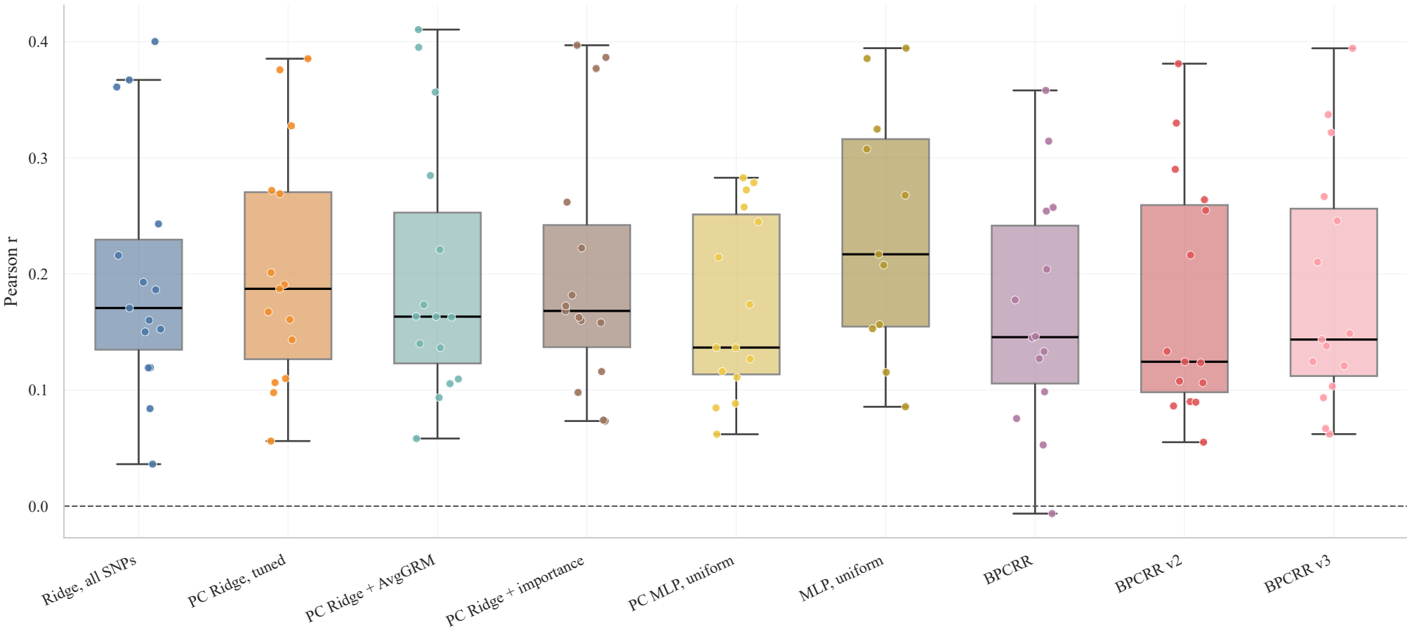
Across-population prediction, Wing length
