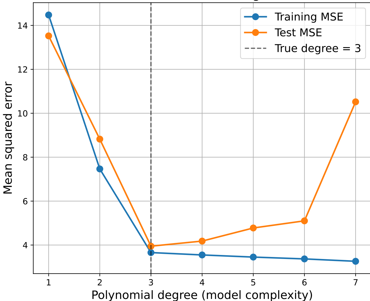
Bias-variance tradeoff: training vs. test error
