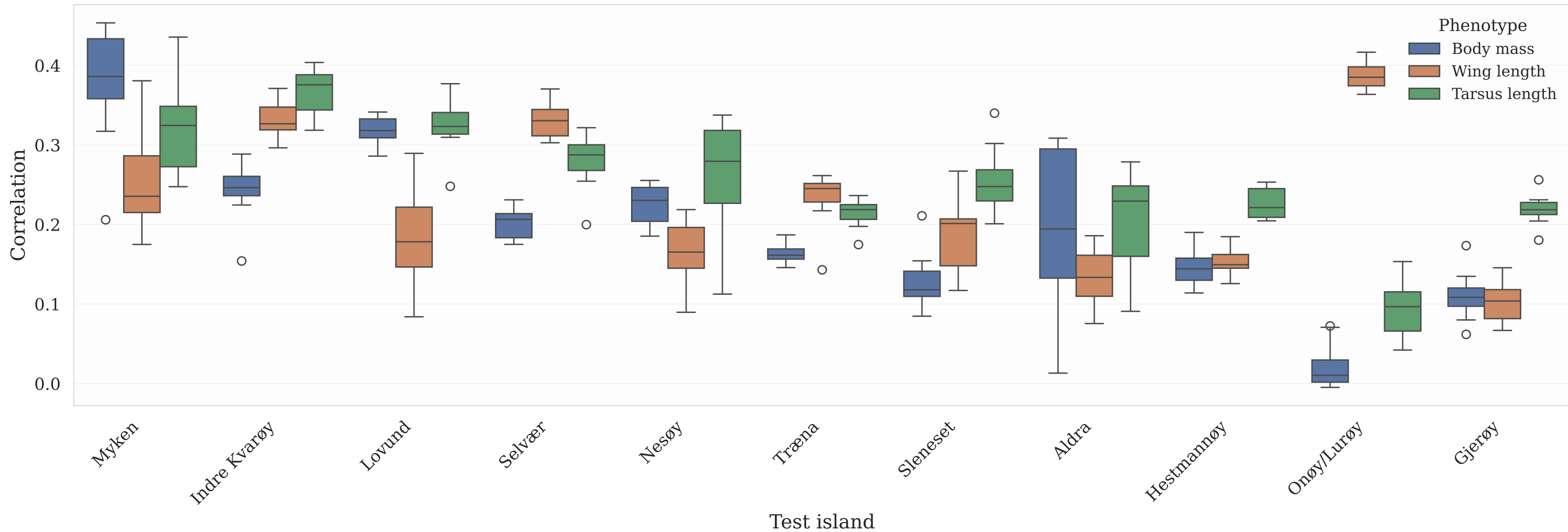
Per-island prediction accuracy by phenotype (grouped by island)
