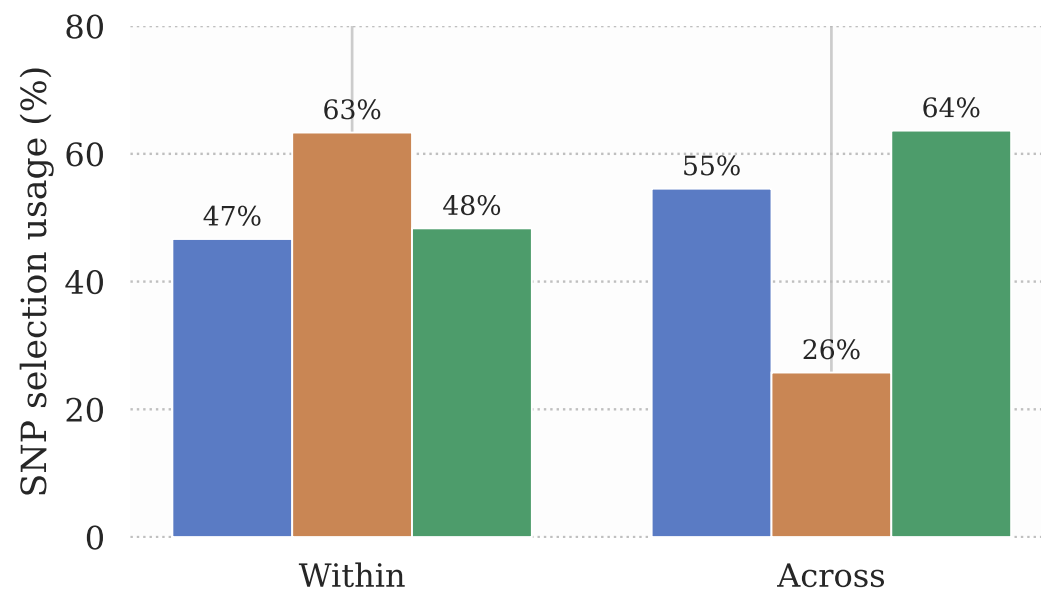
(c) SNPs selected by scenario
