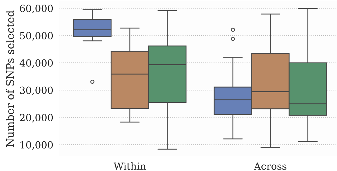
(c) SNPs selected by scenario
