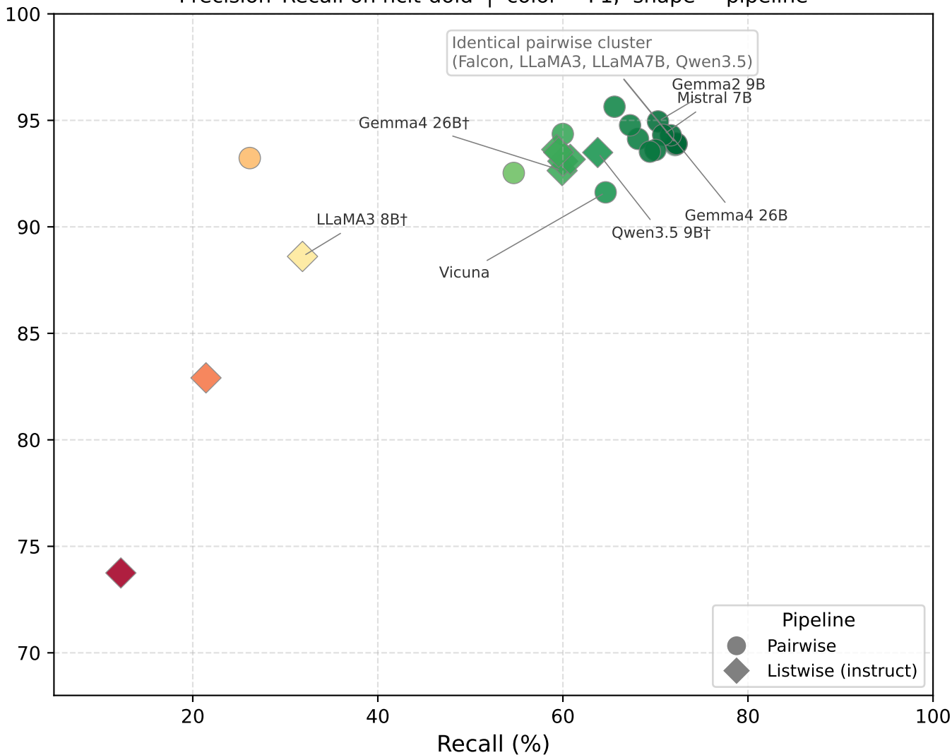
Precision-Recall on ncit-doid | color = F1, shape = pipeline
