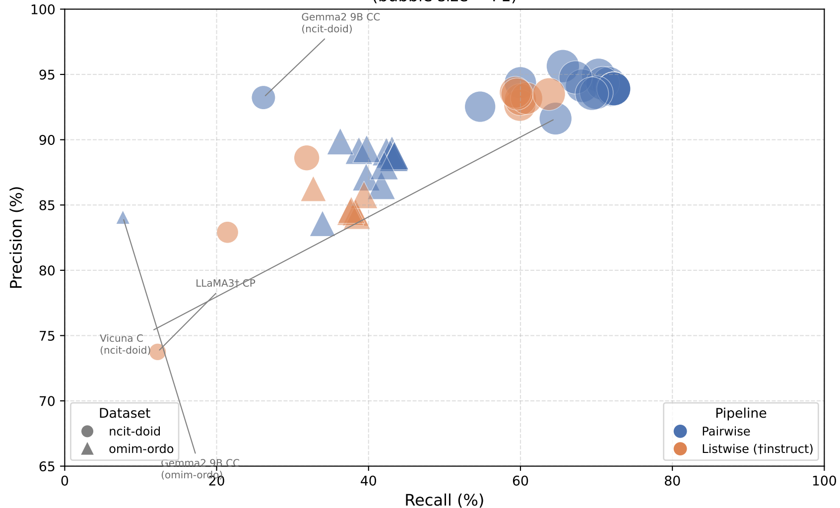
Precision vs. Recall for Pairwise and Listwise LLM Matching (bubble size = F1)
