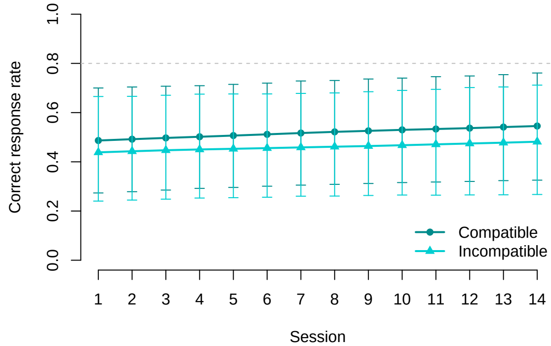
Spin – Splash
