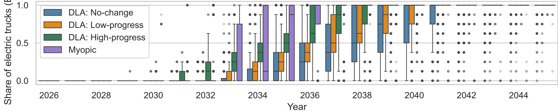
Boxplot for each year, showing BET share in the fleet across 2000 simulation episodes for each strategy.
