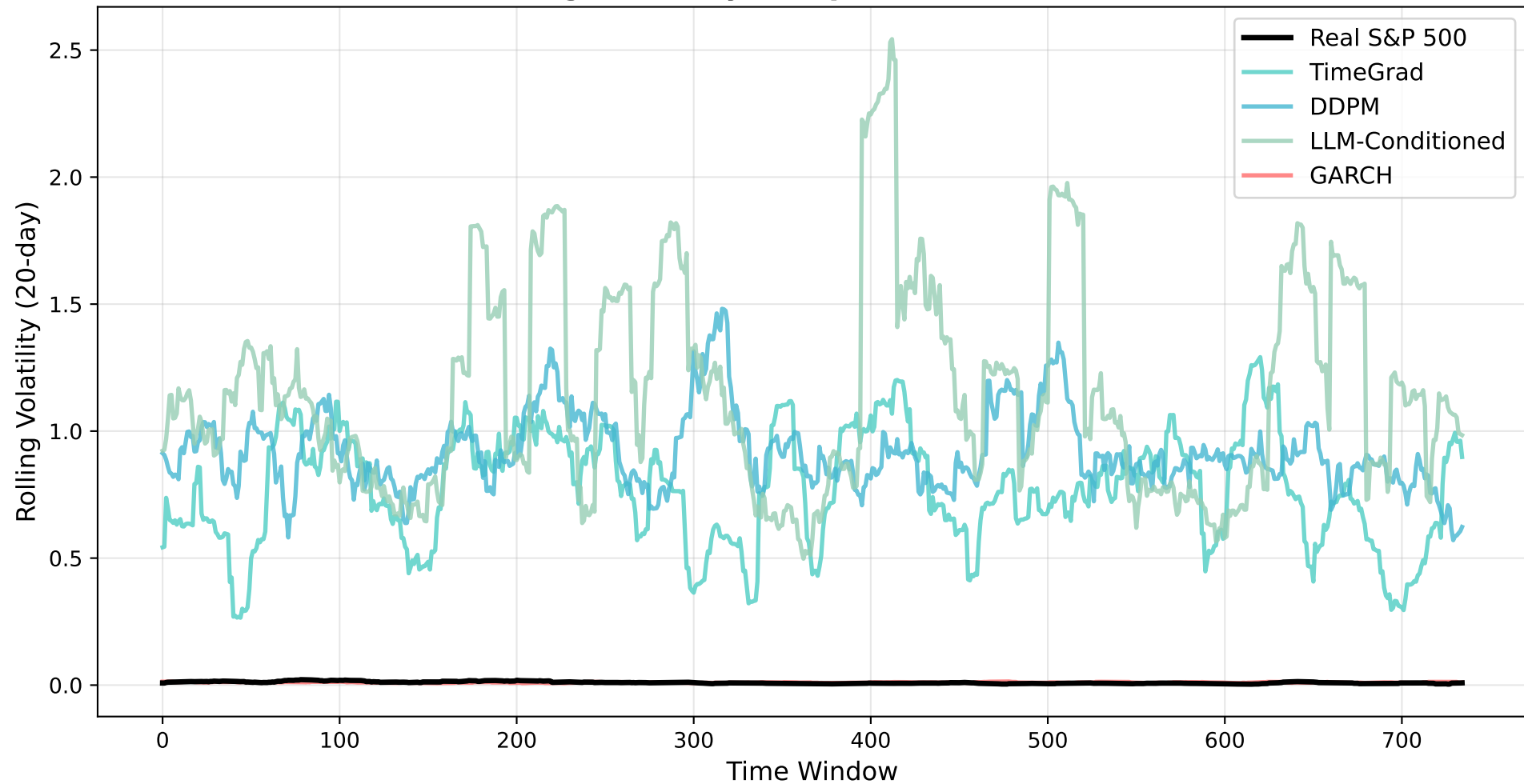
Rolling Volatility Comparison (Corrected)
