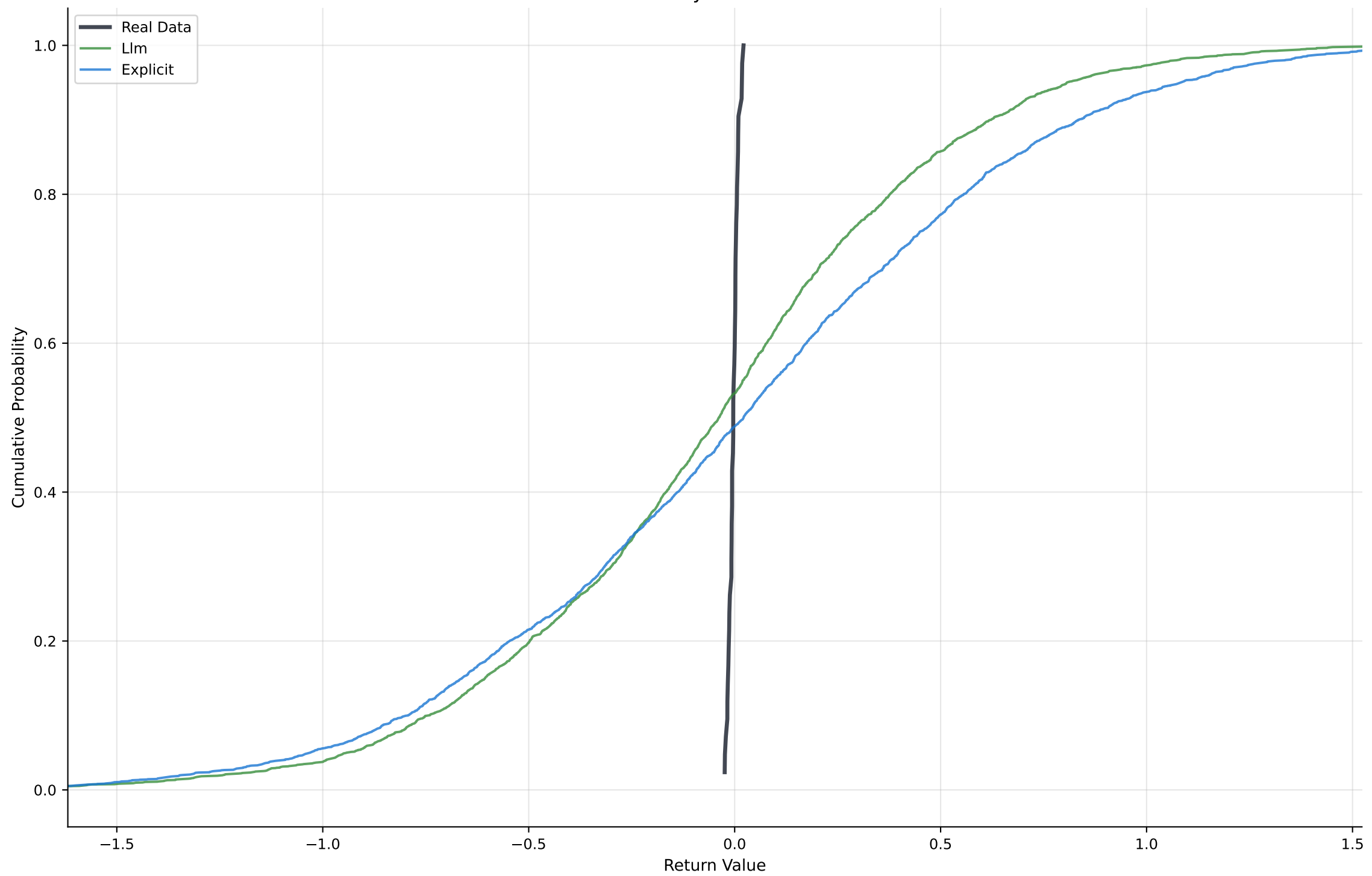
ECDF Overlay - B Covid Crash
