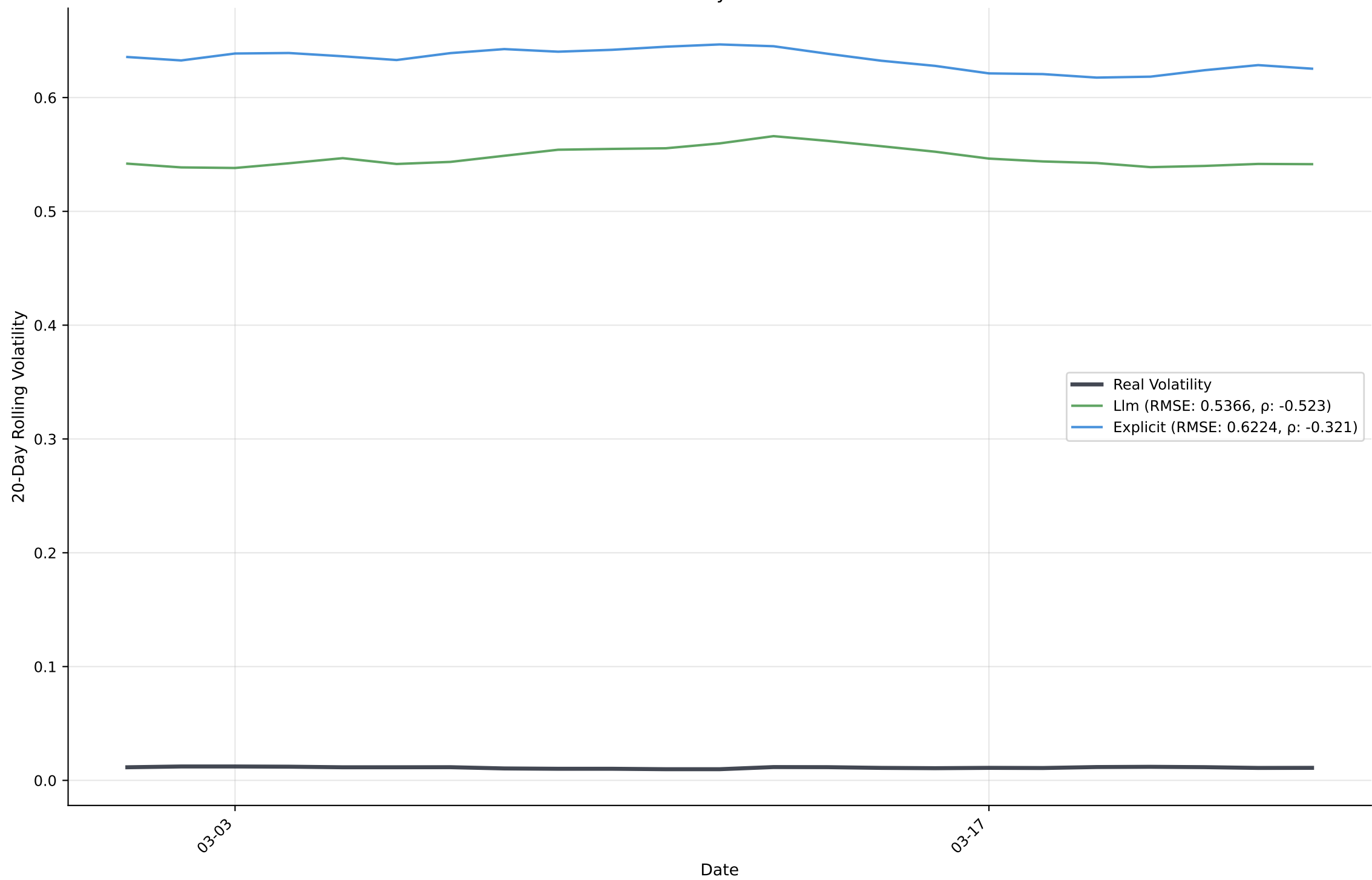
Realized Volatility - B Covid Crash
