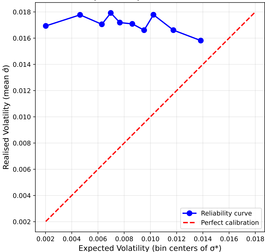
Volatility Reliability Curve (RMSE=0.0096)
