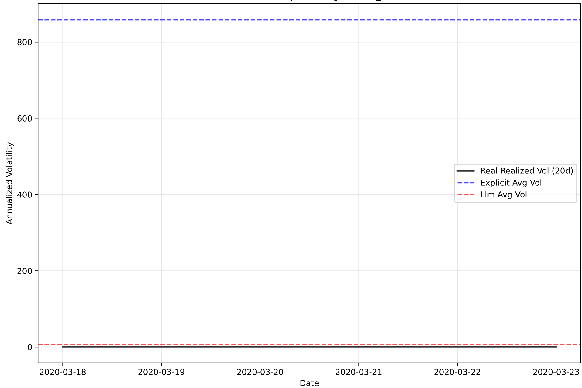
Realized Volatility Tracking - Covid_Crash
