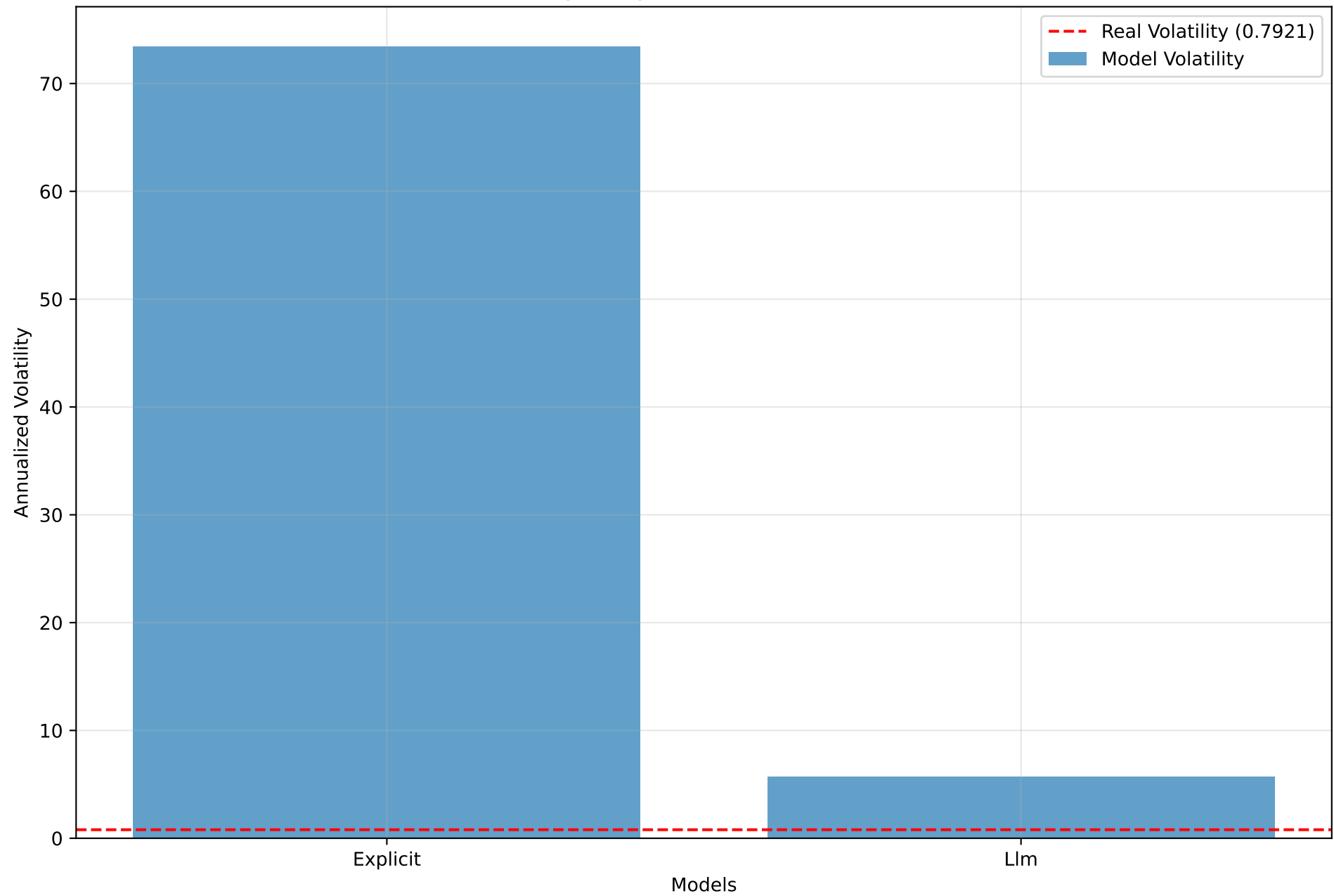
Volatility Comparison - Calm Conditions
