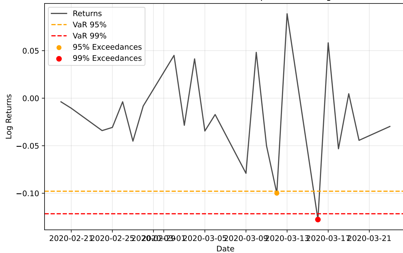
VaR Exceedances - Llm Knob Comp0 Shift+1.0Sigma
