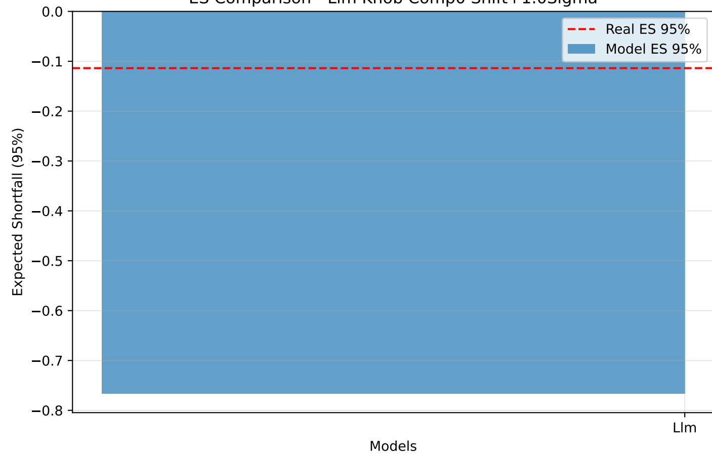
Risk Metrics - Llm Knob Comp0 Shift+1.0Sigma
