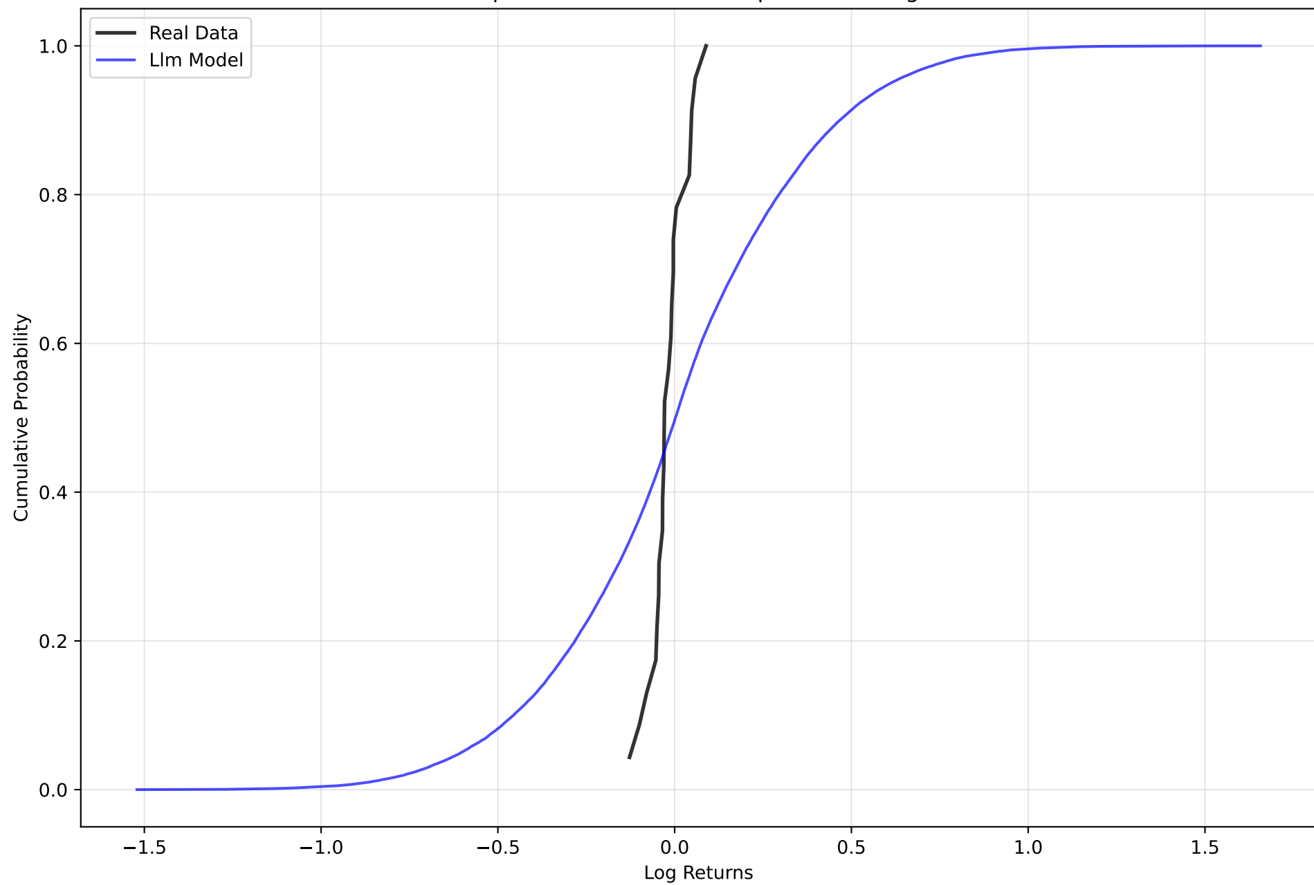
ECDF Comparison - Llm Knob Comp0 Shift 1.0Sigma Mode
